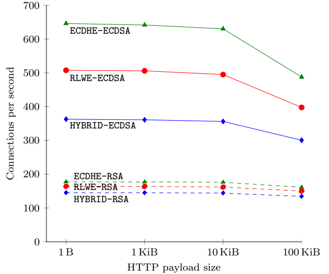
Fig. 1. HTTPS connections per second supported by the server at 128-bit security level. All ciphersuites use AES-128-GCM and SHA256.
